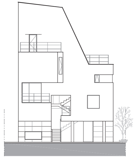
East Elevation
