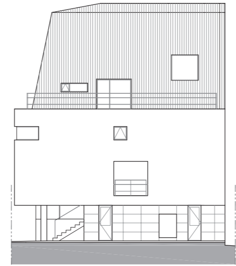
North Elevation
